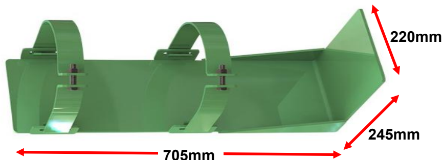
Bracket for 20L, 25L, 30L QTB450-PC
